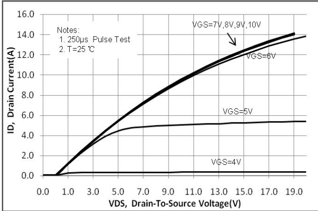
Fig.1. On-state Characteristics
