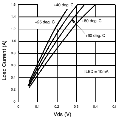
Figure 3. Typical On-Characteristics
