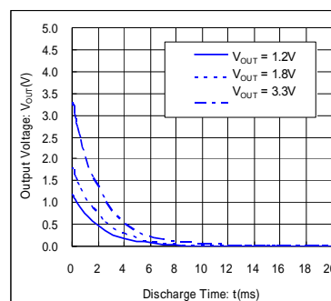
Output Voltage Discharge characteristics R_{DCHG} = 210 (TYP) C_L = 10 \mu\text{F}
