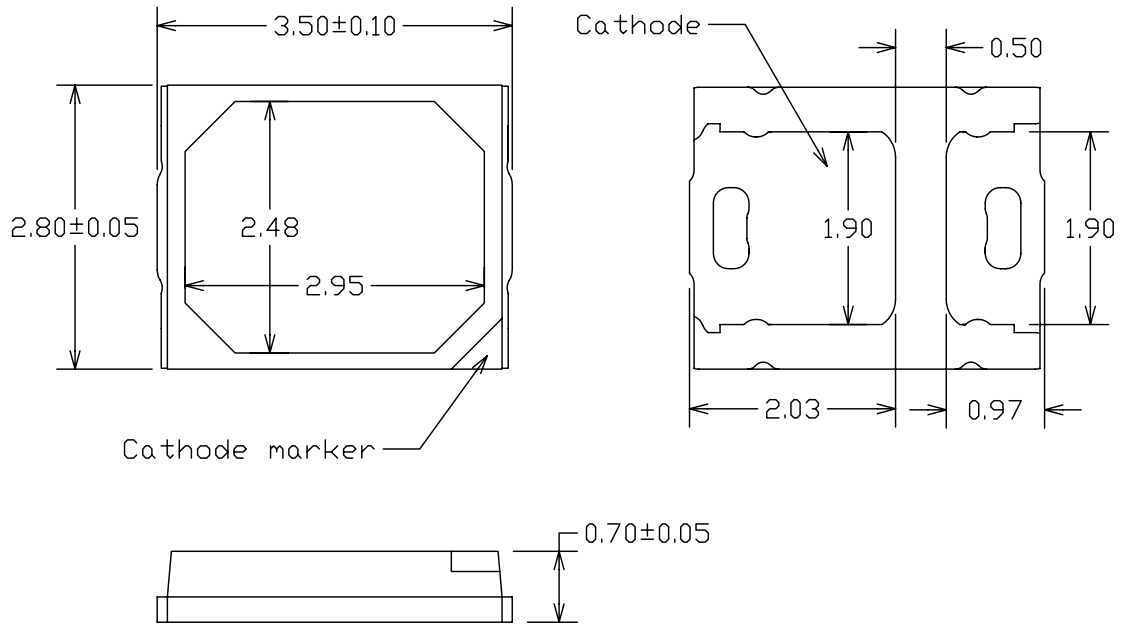
Figure 9. Mechanical dimensions for LUXEON 2835 Line.
