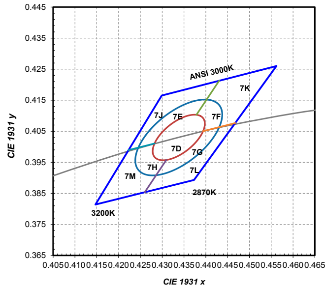
Figure 8c. 1/9 th color bin structure for LUXEON 2835E and LUXEON 2835C 3000K at test current and binning temperatures of T_j=25^\circ\text{C} and T_j=85^\circ\text{C} .
