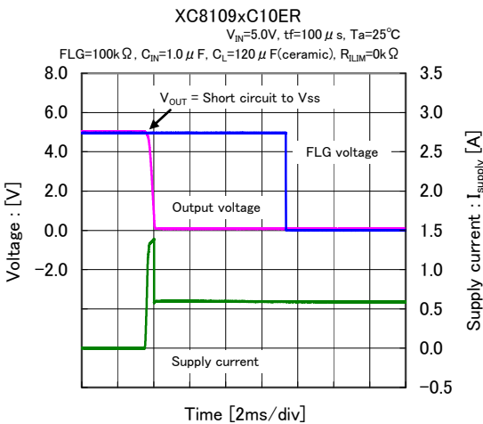
(31) Short-circuit transient response ( V_{OUT} = \text{open} \rightarrow \text{short} , C_L = 120 \mu\text{F} )
