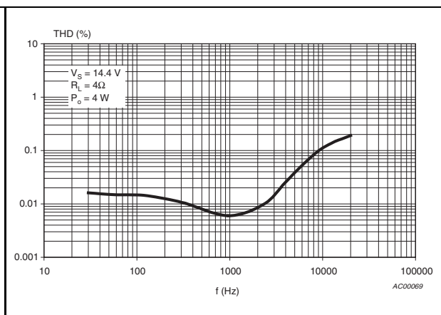
Figure 11. Distortion vs. frequency (RL = 4Ω)
