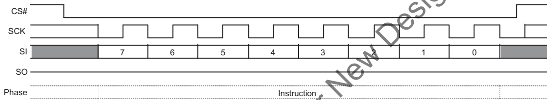
Figure 53. Deep Power-Down Command Sequence
