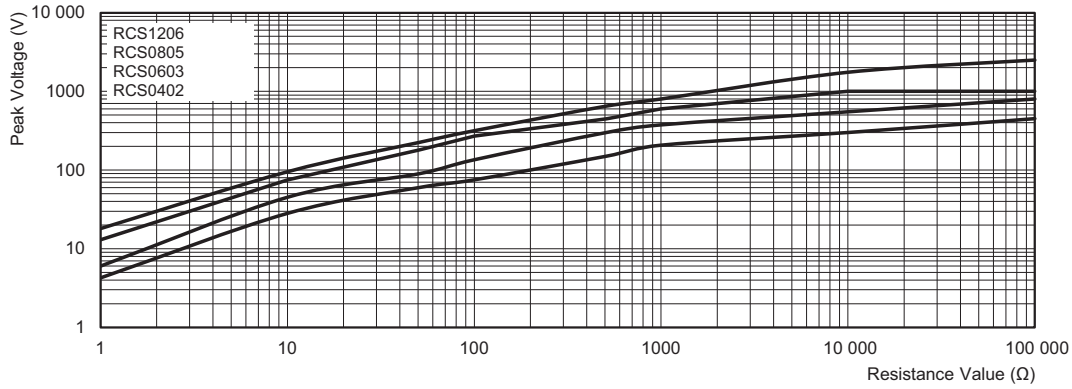
Pulse load rating in accordance with EN 60115-1, 4.27; 1.2 \mu s/50 \mu s; 5 pulses at 12 s intervals; for permissible resistance change 1 %
