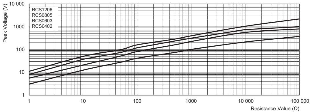
Pulse load rating in accordance with EN 60115-1, 4.27; 10 \mu s/700 \mu s; 10 pulses at 1 min intervals; for permissible resistance change 1 %
