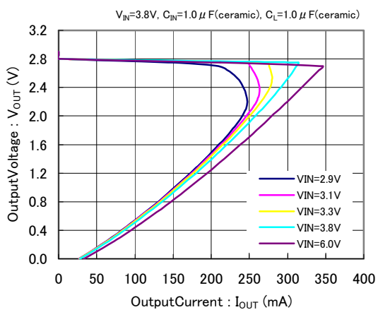
XC6415( V_{OUT}=2.8V )
