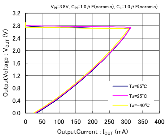
XC6415( V_{OUT}=2.8V )
