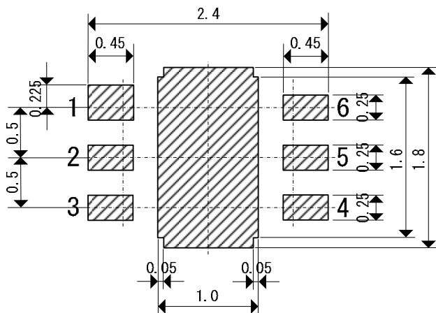
USP-6C Reference Pattern Layout (unit: mm)
