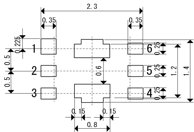
USP-6C Reference Metal Mask Design (unit: mm) (unit: mm)
