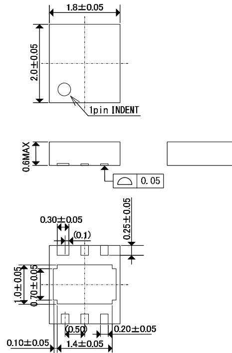
USP-6C (unit: mm)
