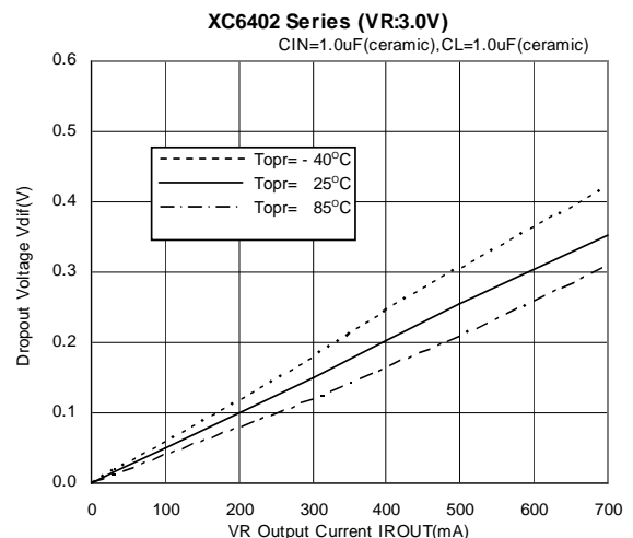
Dropout Voltage vs. VR Output Current
