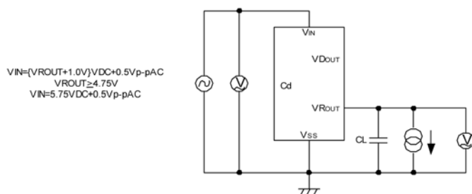
Circuit
