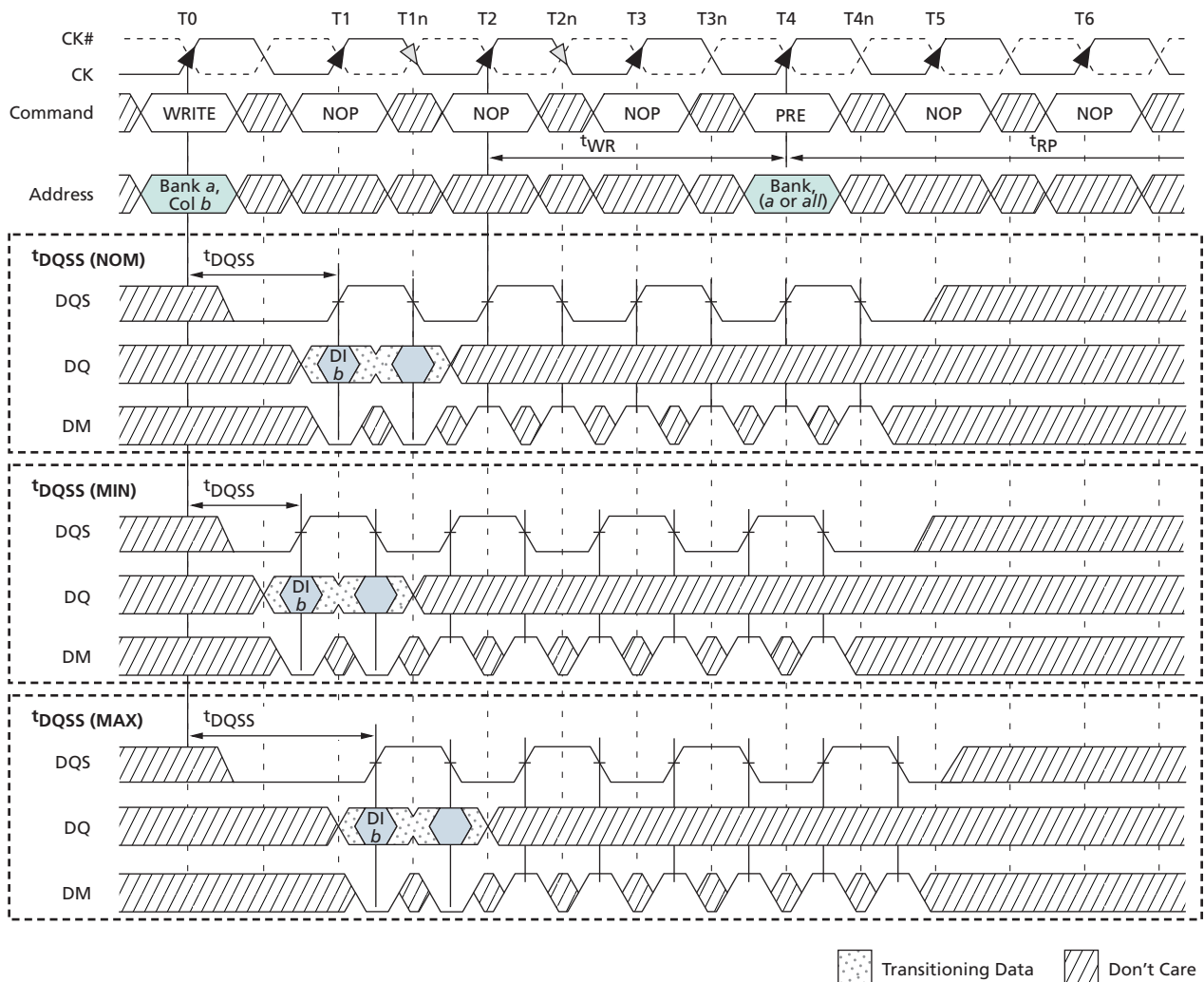
Figure 47: WRITE-to-PRECHARGE – Interrupting
