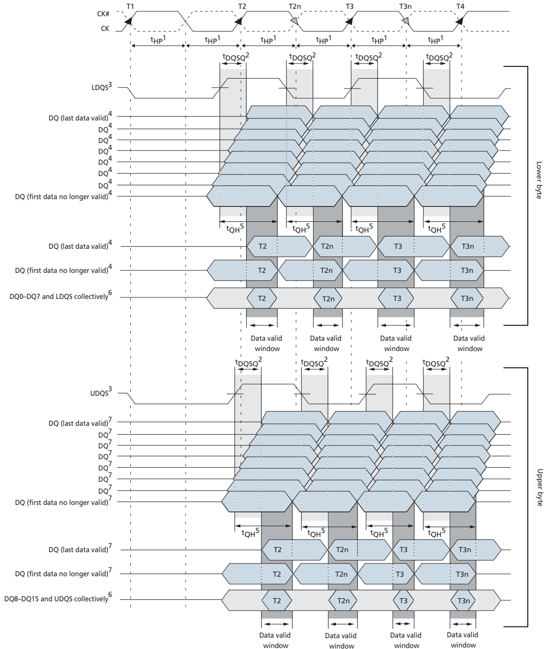
Figure 37: x16 Data Output Timing – t_{DQSQ} , t_{QH} , and Data Valid Window
