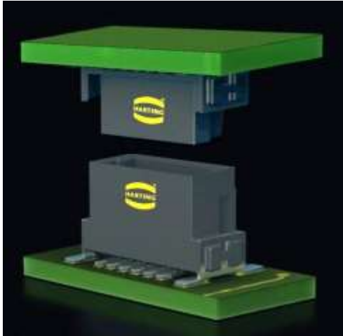
Mezzanine (2 straight connectors)
