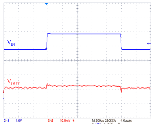
Figure 25. Line transient ( I_{OUT} = 250\text{ mA} )
