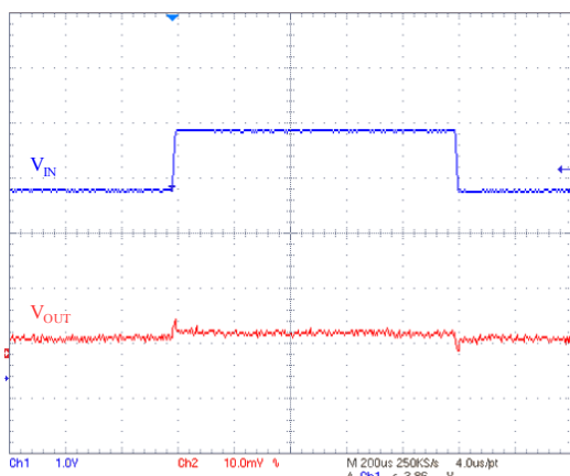
Figure 24. Line transient ( I_{OUT} = 1\text{ mA} )
