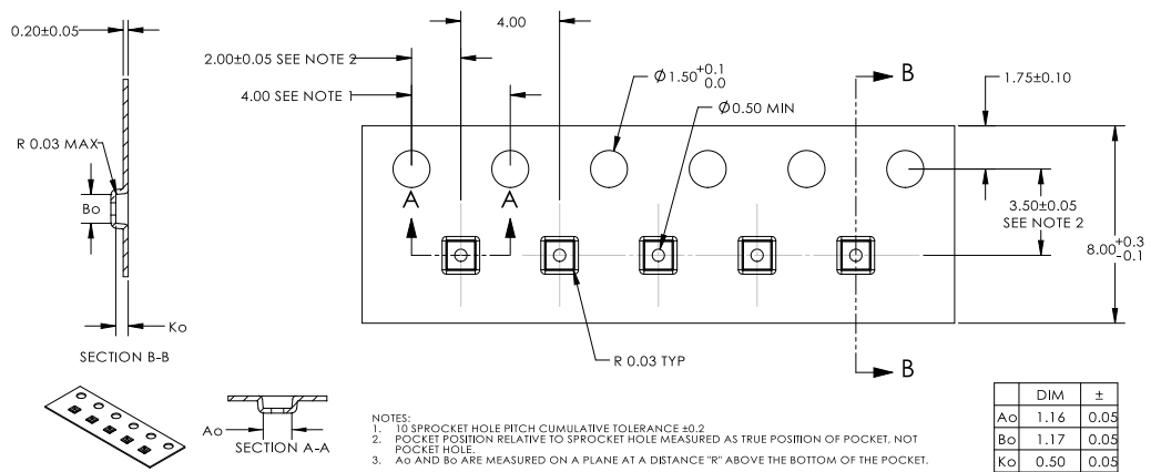
Figure 34. DFN4 (1x1x0.38 pitch 4 mm) carrier tape
