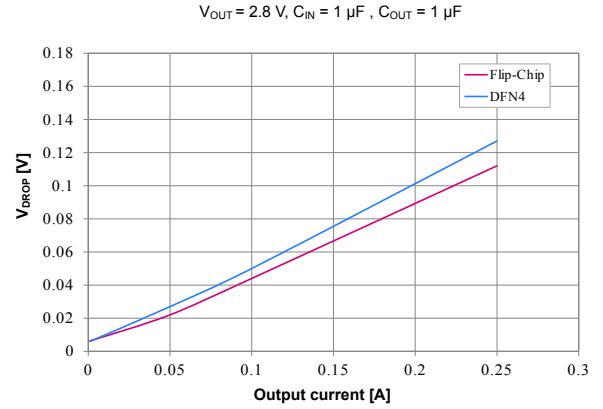
Figure 15. Dropout voltage vs. load current
