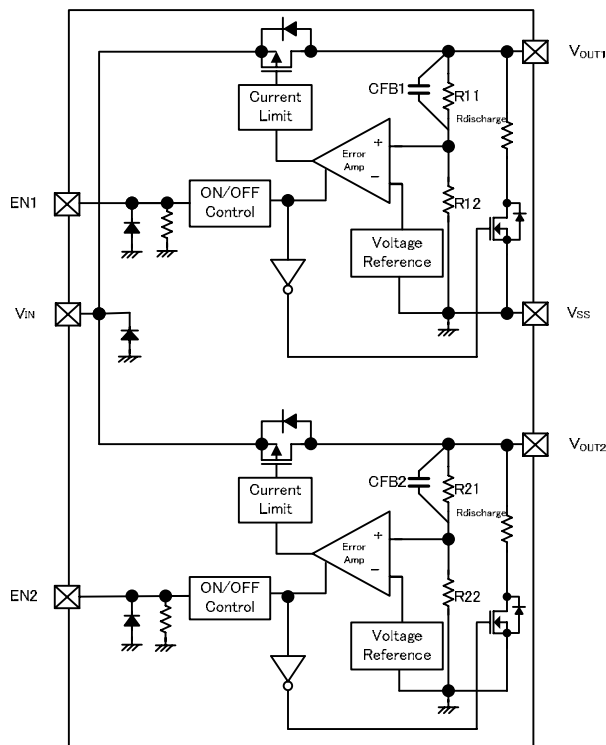
XC6420ABxxxxseries
