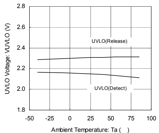
(9) U.V.L.O. Temperature Characteristics XC9220/21 Series
