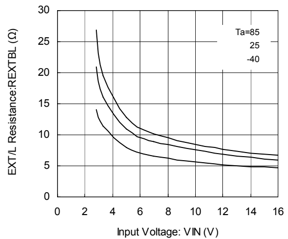
XC9220/21 Series
