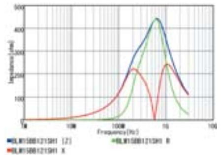
BLM15BB121SZ1/BLM15BB121SH1
