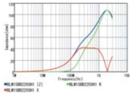
BLM15BB220SZ1/BLM15BB220SH1
