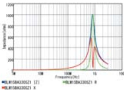
BLM15BA330SZ1
