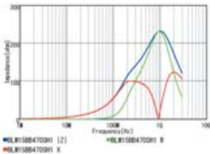
BLM15BB470SZ1/BLM15BB470SH1
