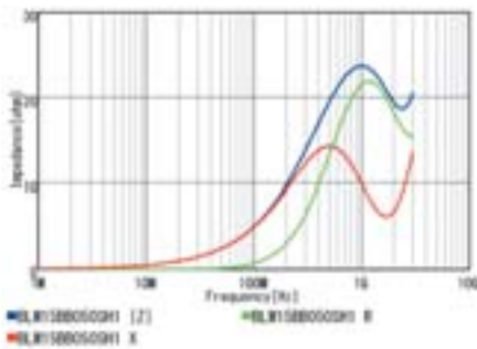
BLM15BB050SZ1/BLM15BB050SH1
