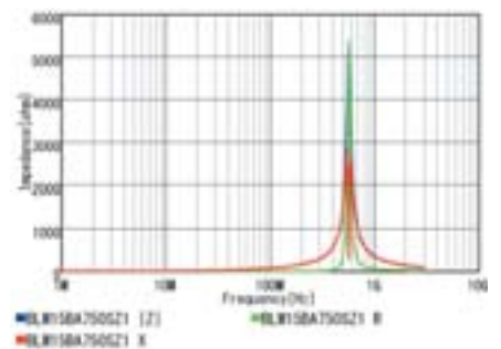
BLM15BA750SZ1
