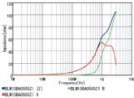
BLM15BA050SZ1
