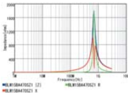
BLM15BA470SZ1
