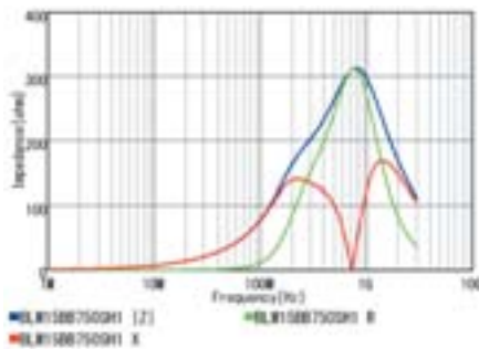
BLM15BB750SZ1/BLM15BB750SH1
