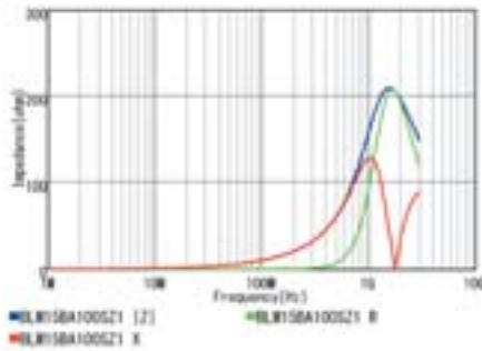
BLM15BA100SZ1
