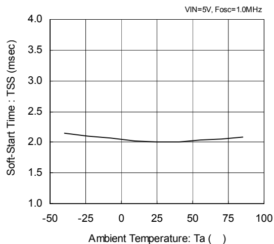
XC9220/21 Series
