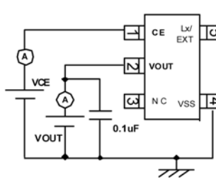
Circuit ⑥
