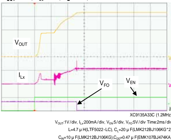
(30) Soft-start
