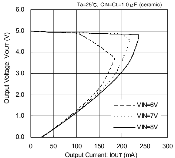
XC6216B/D 502
