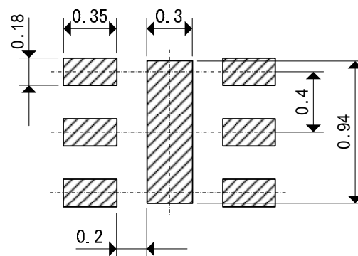
USP-6B04 Reference Pattern Layout
