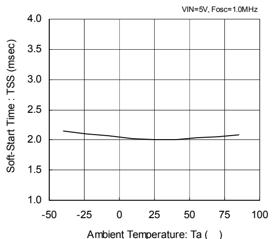
XC9220/21 Series
