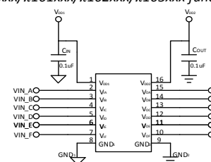
Figure 2. \pi 160xxx Typical Application Circuit
