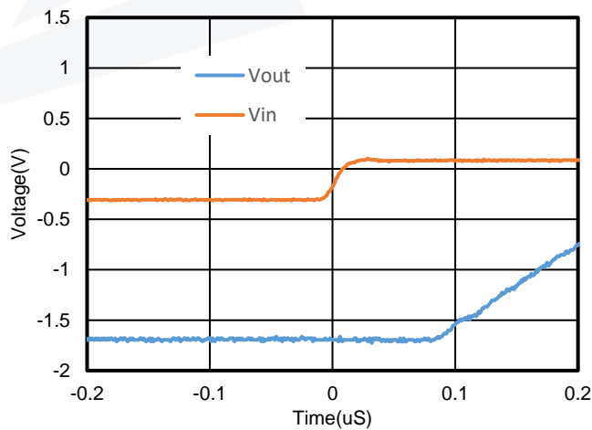
Figure 11. Positive Overload Recovery, V S = 3.3V, V CM = 1.65V, G = 11
