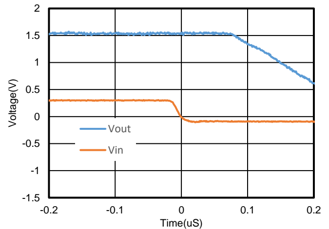
Figure 12. Negative Overload Recovery, V S = 3.3V, V CM = 1.65V, G = 11
