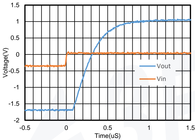
Figure 9. Positive Settling Time, V S = 3.3V, V CM = 1.65V, G = 11
