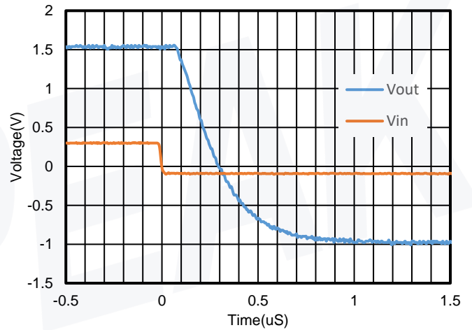
Figure 10. Negative Settling Time, V S = 3.3V, V CM = 1.65V, G = 11
