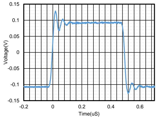
Figure 8. Small Signal Step Response, G = 1, R L = 10k \Omega , C L = 100pF
