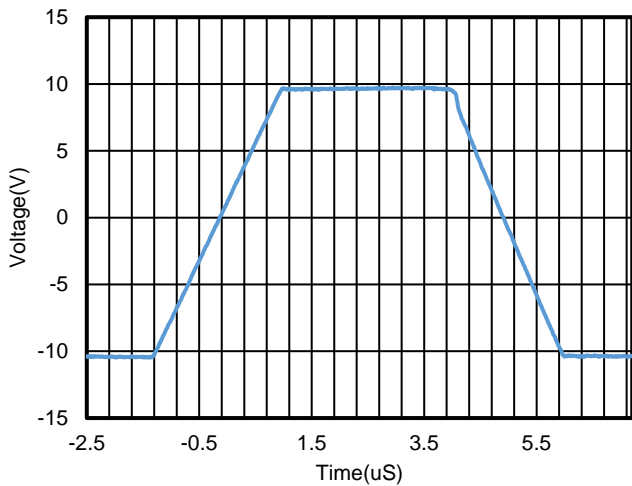
Figure 7. Large Signal Step Response, G = 1, R L = 10k \Omega , C L = 100pF
