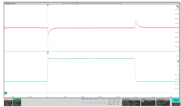
Figure 20. Load Transient
