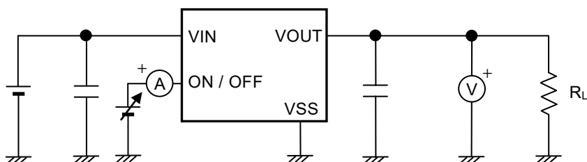
Figure 9 Test Circuit 3
