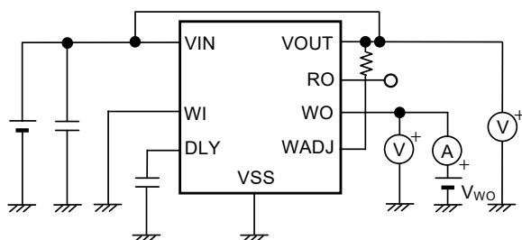
Figure 29 Test Circuit 11
