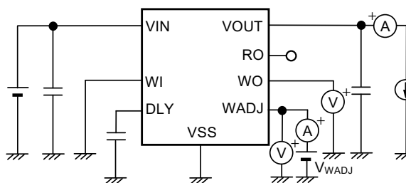
Figure 25 Test Circuit 7
