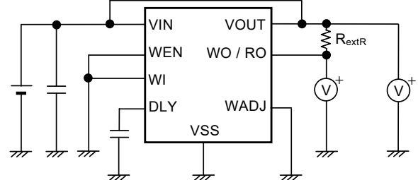
Figure 12 Test Circuit 4
