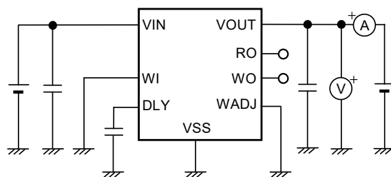
Figure 20 Test Circuit 2
