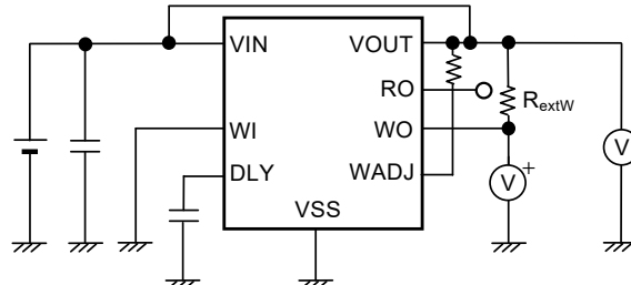
Figure 28 Test Circuit 10
