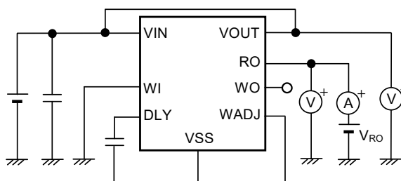
Figure 23 Test Circuit 5
