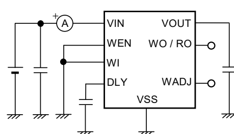
Figure 18 Test Circuit 10
