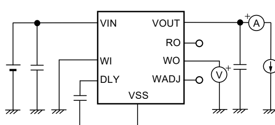
Figure 24 Test Circuit 6
