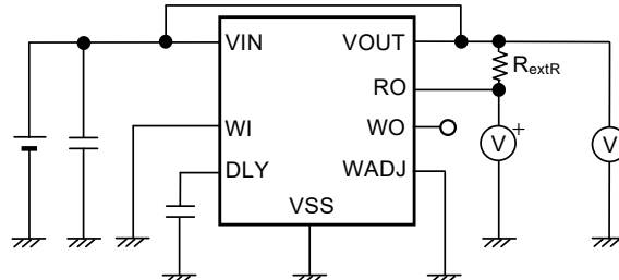
Figure 22 Test Circuit 4
