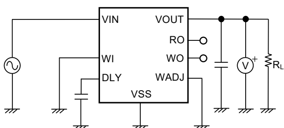
Figure 21 Test Circuit 3
