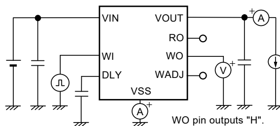
Figure 26 Test Circuit 8
