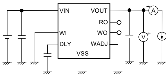
Figure 19 Test Circuit 1
