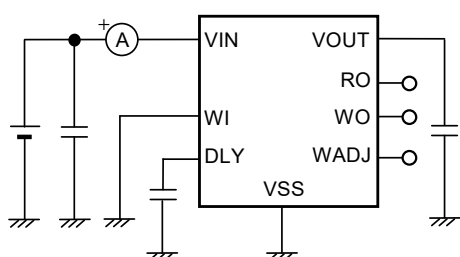
Figure 27 Test Circuit 9
