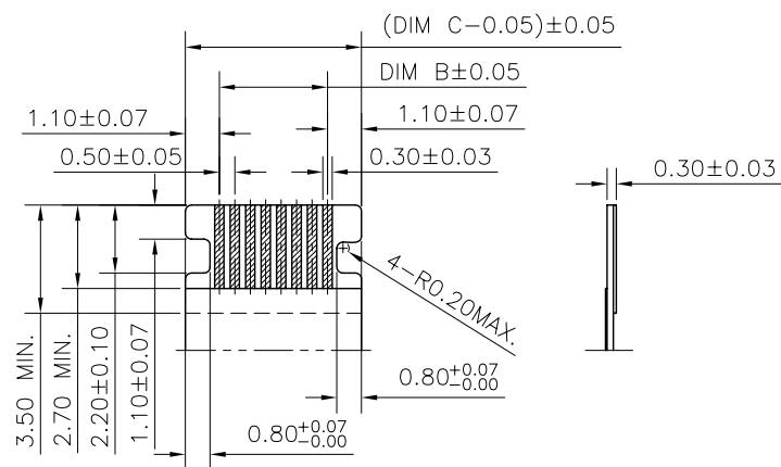
RECOMMENDED FPC/FFC DIMENSIONS GENERAL TOLERANCE ±0.05
