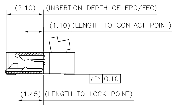
SECTION A-A SCALE 6:1
