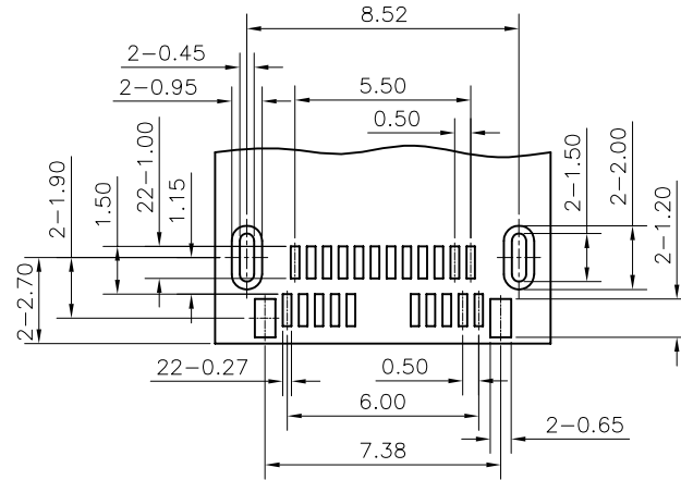
RECOMMENDED PCB DIMENSIONS (REF.) GENERAL TOLERANCE \pm 0.05
