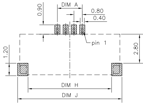
RECOMMENDED PCB LAYOUT GENERAL TOLERANCE \pm 0.05
