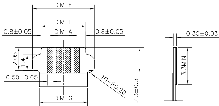
RECOMMENDED FPC/FFC DIMENSIONS GENERAL TOLERANCE \pm 0.05
