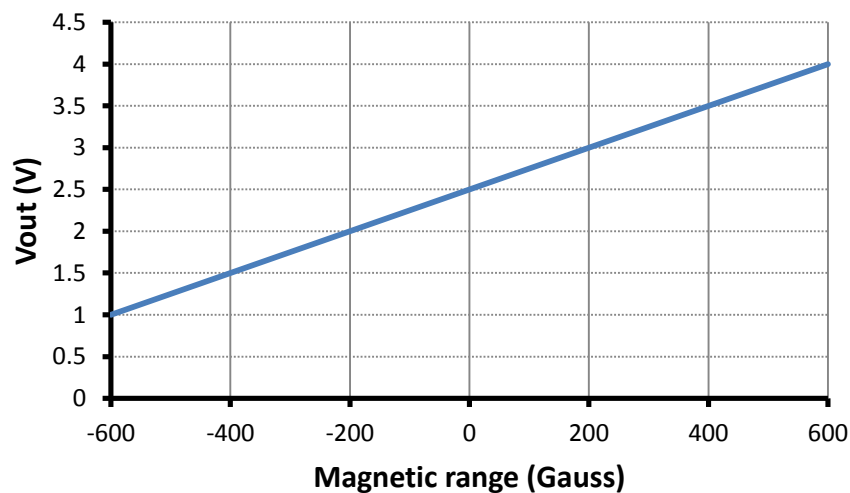
Magnetic range VS Vout @25 ° C
