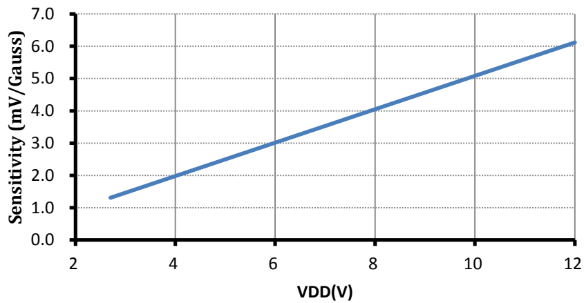
Sensitivity VS VDD @25 °C
