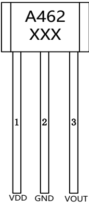
TO92S
