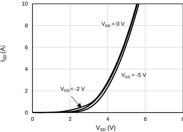
Figure 10: Body Diode Characteristics at 175°C
