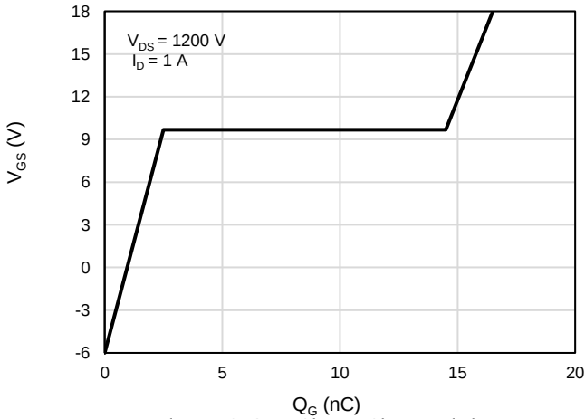
Figure 12: Gate-Charge Characteristics
