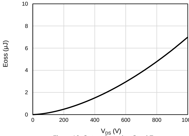
Figure 16: Output Capacitor Stord Energy
