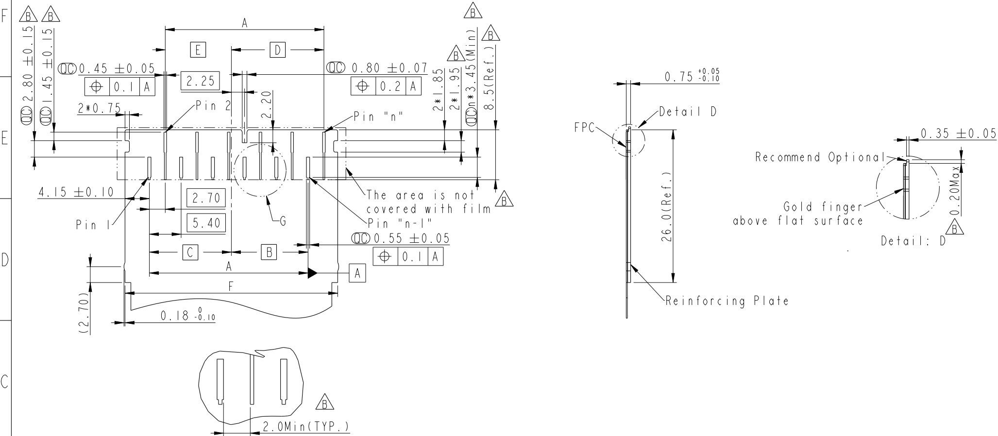
RECOMMENDED FPC LAYOUT
