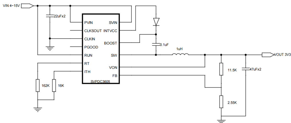
Scheme diagram of high efficiency 1MHz, 5A buck regulator
