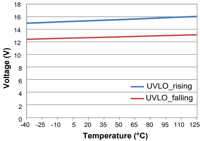
Figure 2. UVLO vs. Temperature
