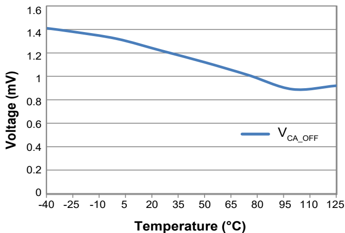
Figure 6. V_{CA\_OFF} vs. Temperature
