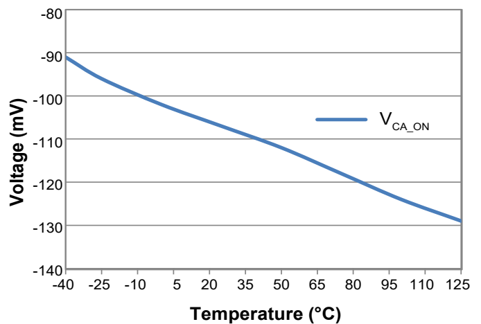
Figure 5. V_{CA\_ON} vs. Temperature
