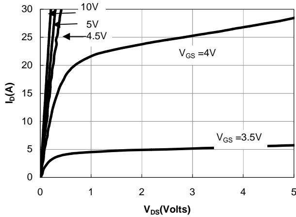
Figure 1: On-Regions CharacteristicCS
