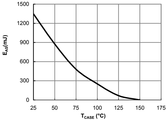
Figure 12: Avalanche energy
