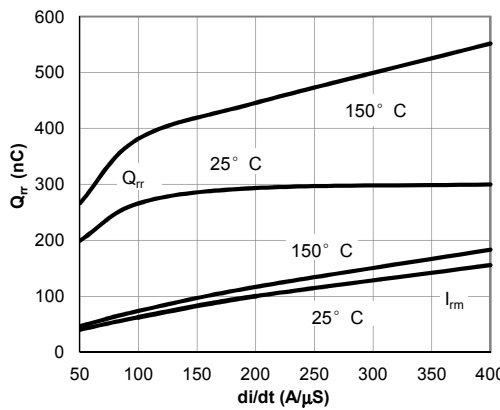
Figure 23: Diode Reverse Recovery Charge and Peak Current vs. di/dt ( V_{GE}=15V, V_{CE}=400V, I_F=7A )
