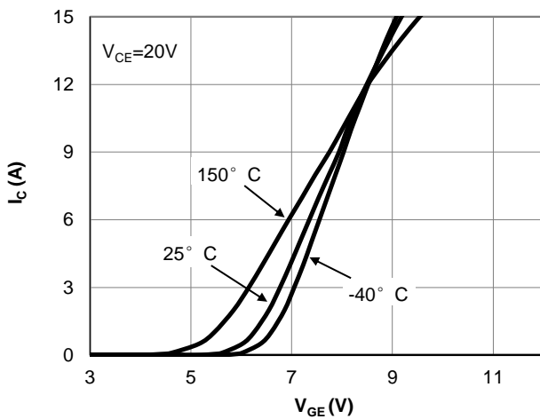
Figure 3: Transfer Characteristic
