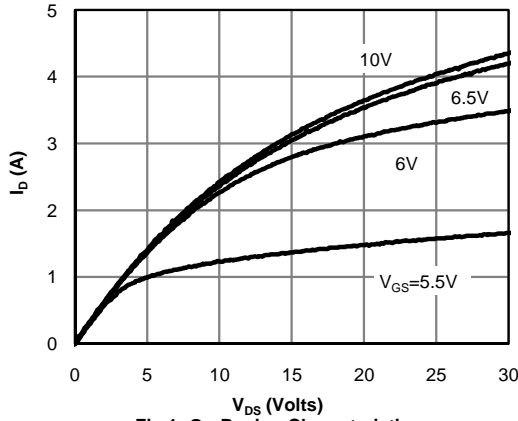
Fig 1: On-Region Characteristics
