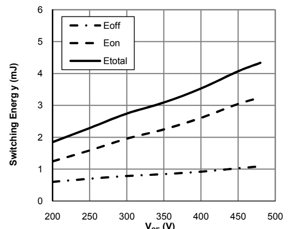
Figure 18: Switching Loss vs. V_{CE} ( T_J=150^\circ\text{C}, V_{GE}=15\text{V}, I_C=50\text{A}, R_g=6\Omega )
