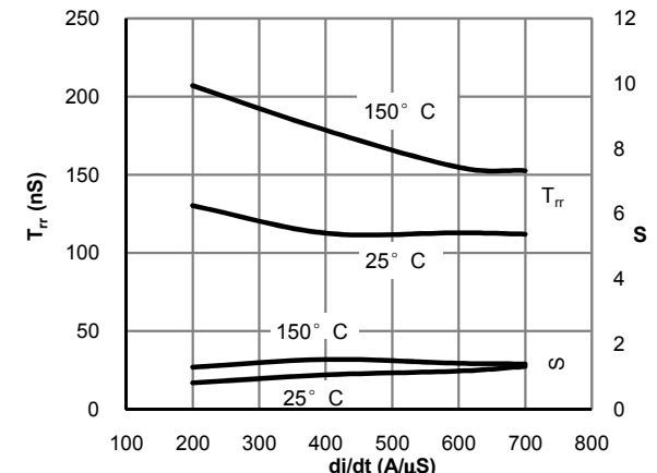
Fig 24: Diode Reverse Recovery Time and Softness Factor vs. di/dt ( V_{GE}=15V, V_{CE}=400V, I_F=25A )
