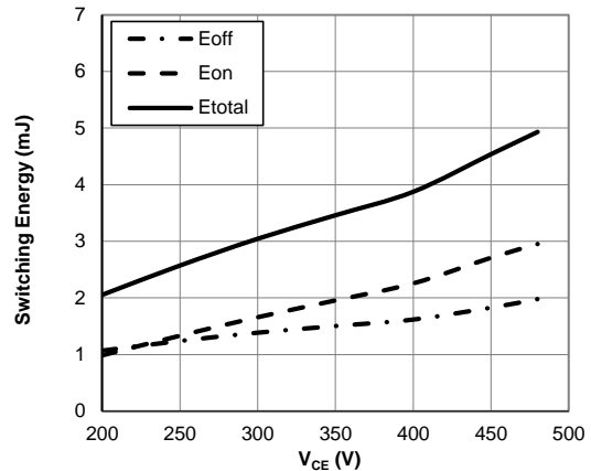
Figure 20: Switching Loss vs. V_{CE} ( T_j=175^\circ C, V_{GE}=15V, I_C=60A, R_g=5\Omega )
