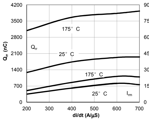
Fig 23: Diode Reverse Recovery Charge and Peak Current vs. di/dt ( V_{GE}=15V, V_{CE}=400V, I_f=60A )
