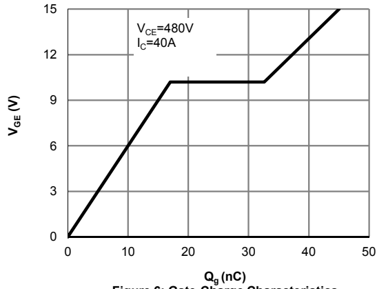
Figure 6: Gate-Charge Characteristics
