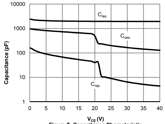
Figure 7: Capacitance Characteristic
