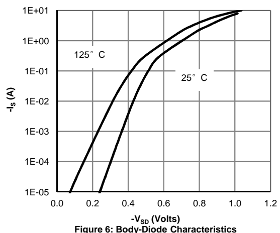
Figure 6: Body-Diode Characteristics
