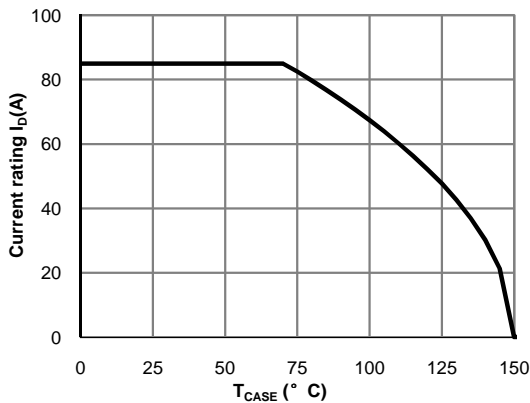
Figure 14: Current De-rating (Note C)
