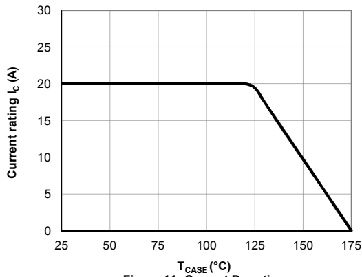
Figure 11: Current De-rating
