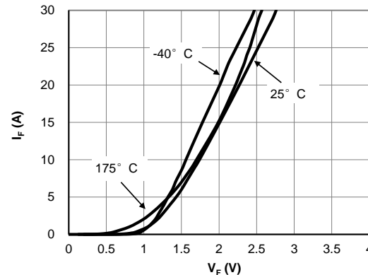
Figure 4: Diode Characteristic
